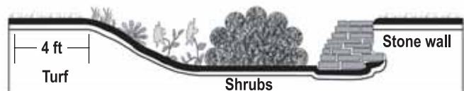
Asymmetrical raingarden with masonry wall
